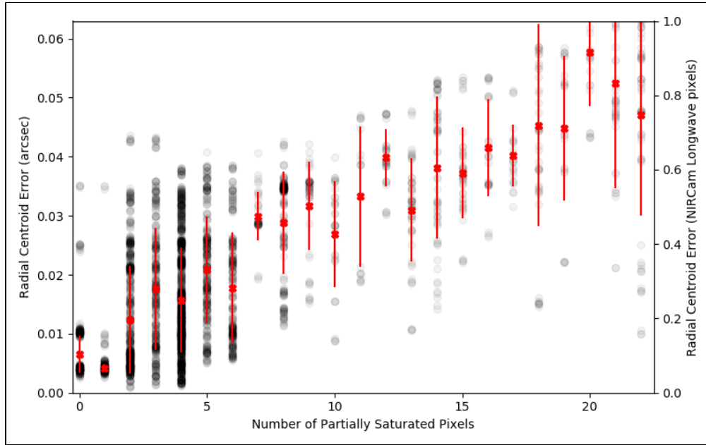
Figure 5. Centroiding error versus the number of partially saturated pixels.
