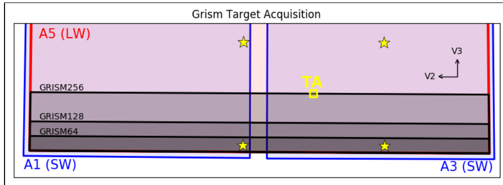
Figure 1. Target acquisition for grism time-series observations
