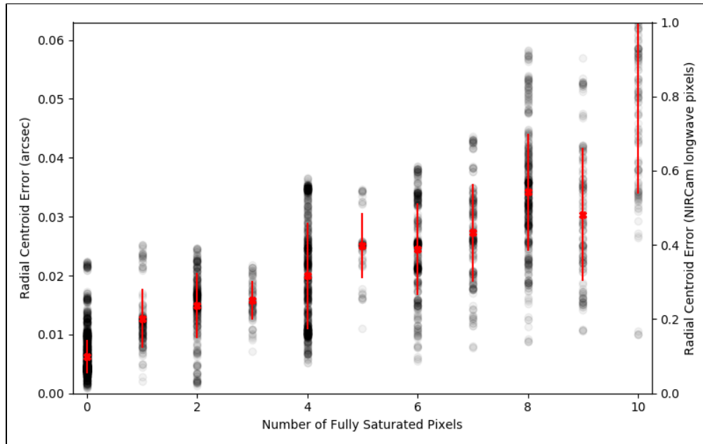
Figure 4. Centroiding error versus the number of fully saturated pixels.
