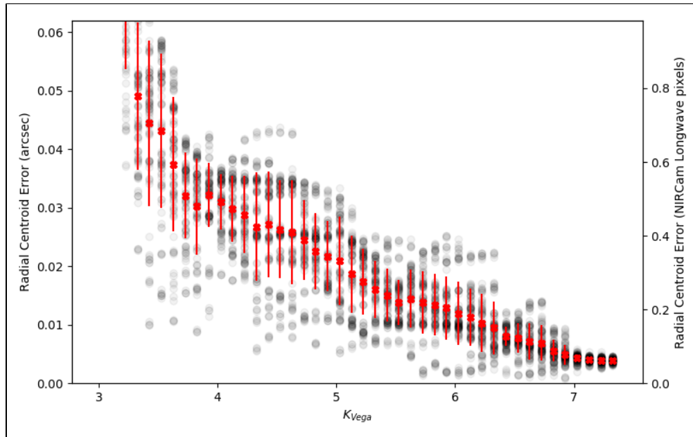
Figure 3. Centroiding error versus source brightness
