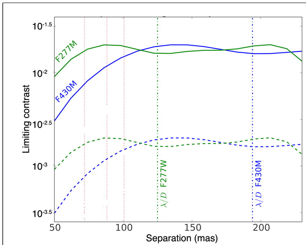
Example of estimating HCI limiting performance for NIRISS/AMI. Adapted from Figure 16 in Greenbaum et al. (2015) .
